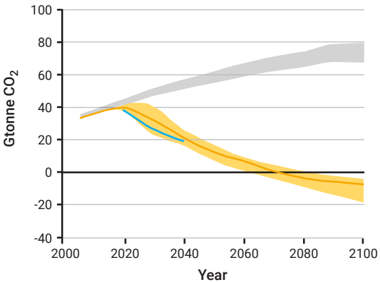
Global CO 2 emissions
