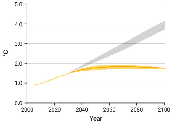
Global mean temperature increase
