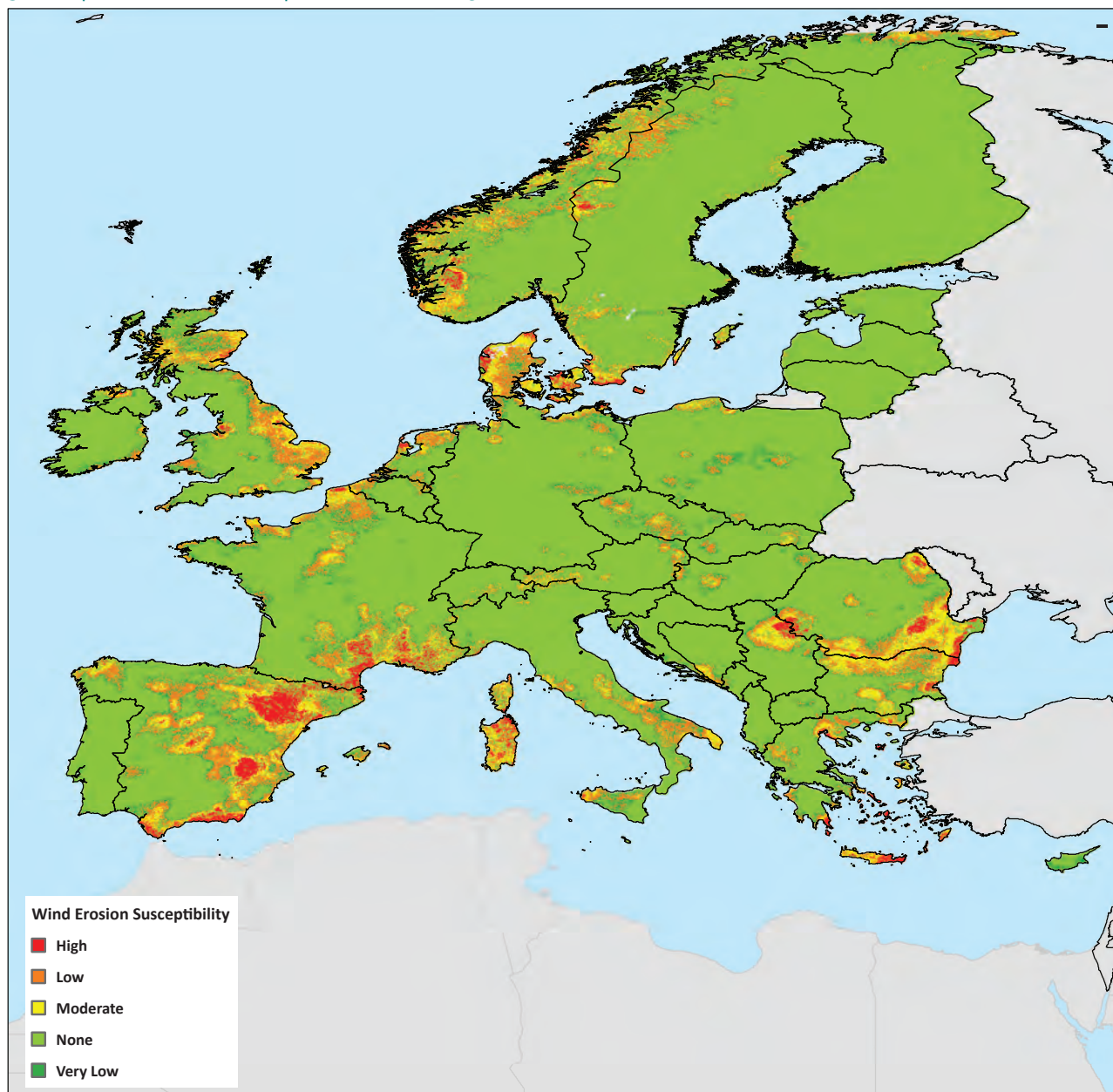
Figure-L2 45: Wind erosion susceptibility in Europe using the index of Land Susceptibility to Wind Erosion (ILSWE) predicted for 36 European countries (at a spatial resolution of 500m)
