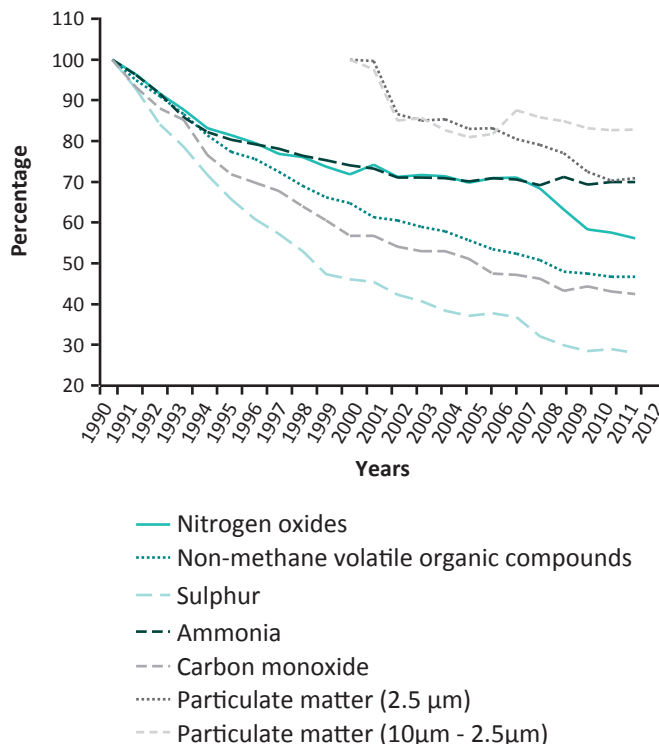
Figure 2.3.2: Emission trends in the ECE region (excluding Canada and the United States of America)
