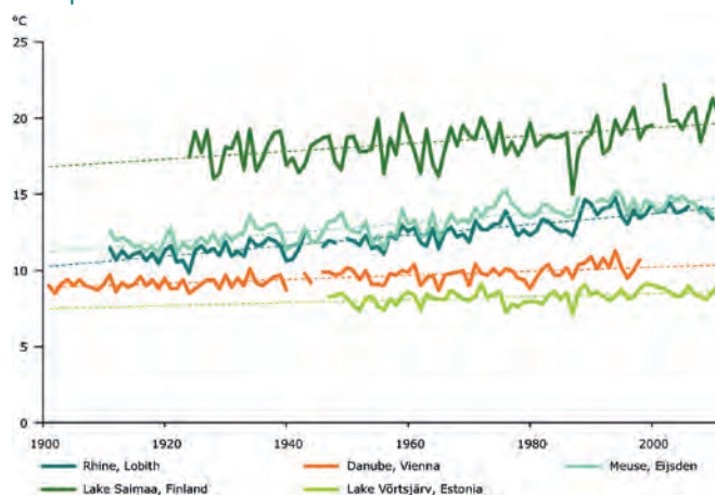
Figure-L2 33: Trends in water temperature of large European rivers and lakes
