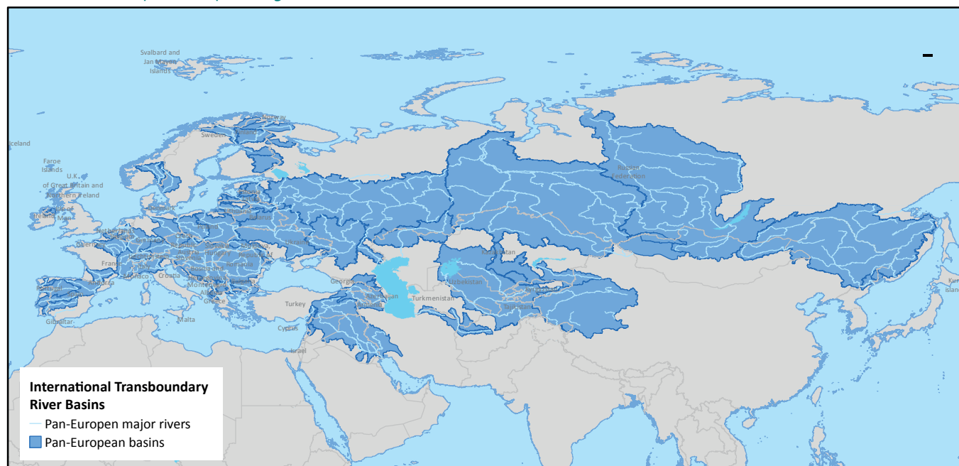
Figure-L2 35: Map juxtaposing national borders of the 54 countries on international river basins. There are 147 international river basins in the pan-European region, 12 of which are lakes
