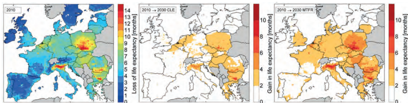
Figure 4.2.10: Current (2010) and projected (2030) effects of air pollution on life expectancy in the EU
