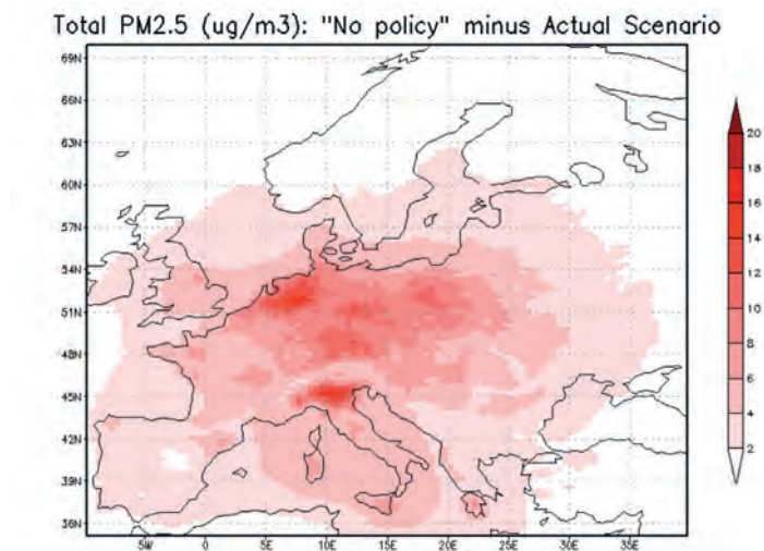
Figure-L2 18: No policy scenario minus the actual scenario. The darker the red colour, the larger the air pollution reductions
