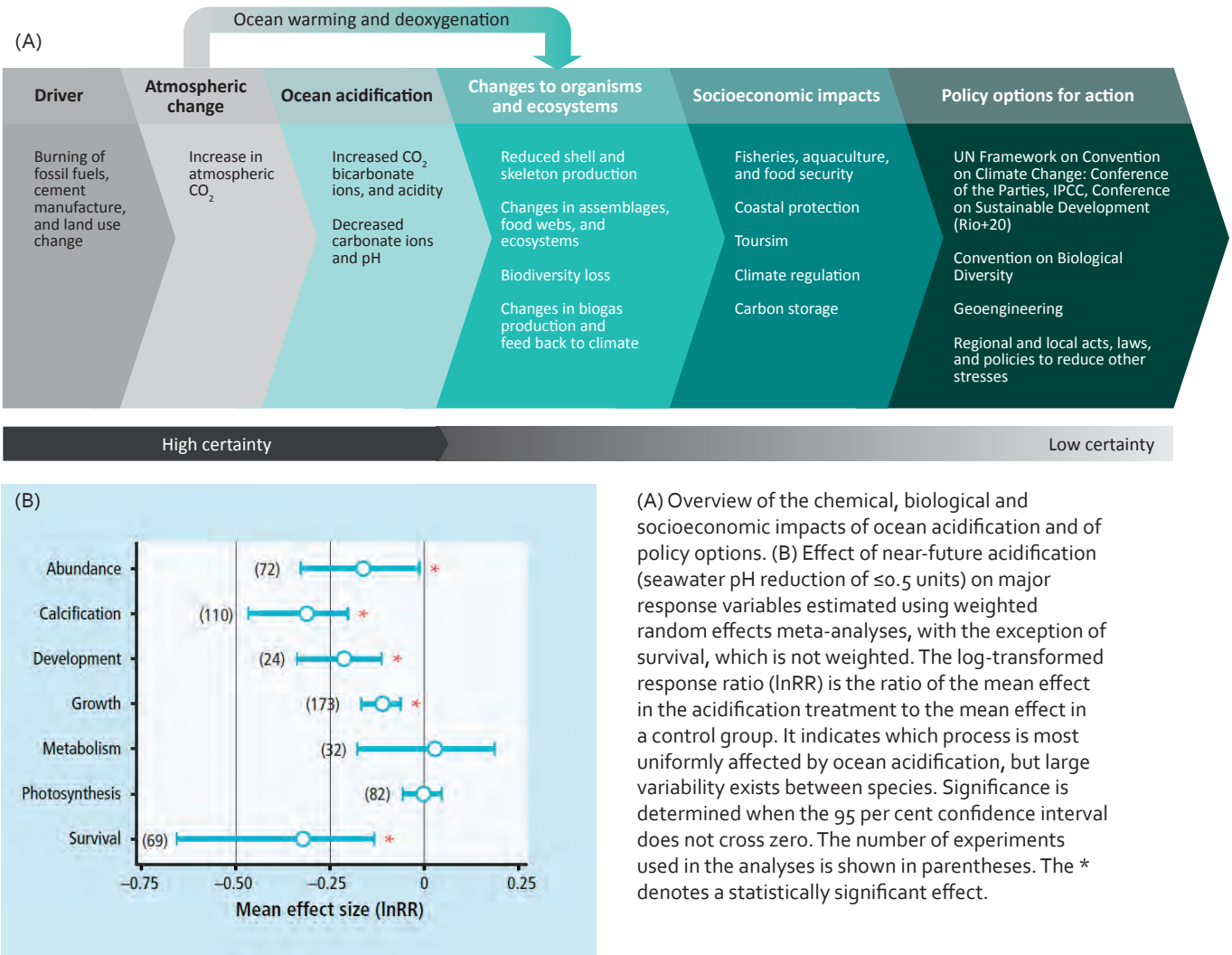
Figure-L2 40: Ocean acidification
